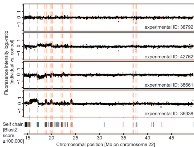
Fig. 1. Association of breakpoints and SDs. Genomic locations of SDs are indicated by BlastZ (32) self-chain matches to the human reference sequence (black vertical bars). SDs coinciding with deletion/duplication breakpoints are highlighted by a red dashed line. The association of breakpoints and SDs [consistent with earlier observations (1, 2, 9, 16, 22)] indicates that nucleotide sequence signatures can facilitate breakpoint mapping.
