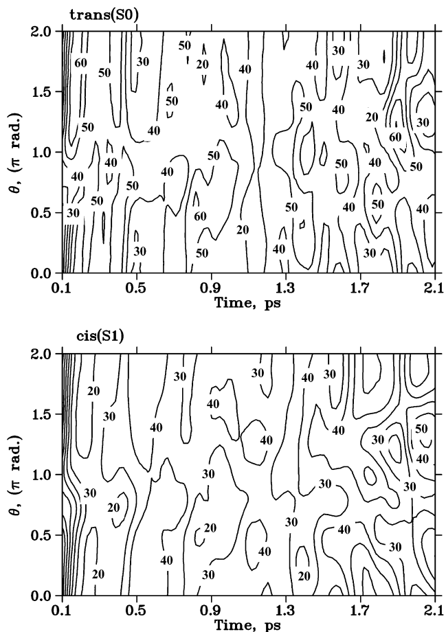
Figure 3. Contour plots of trans- S_0 (upper panel) and cis- S_1 (lower panel) time-dependent percentage populations for bichirped coherent control of rhodopsin as a function of the relative phase \theta = \theta_1 - \theta_2 of the photoexcitation pulses.
