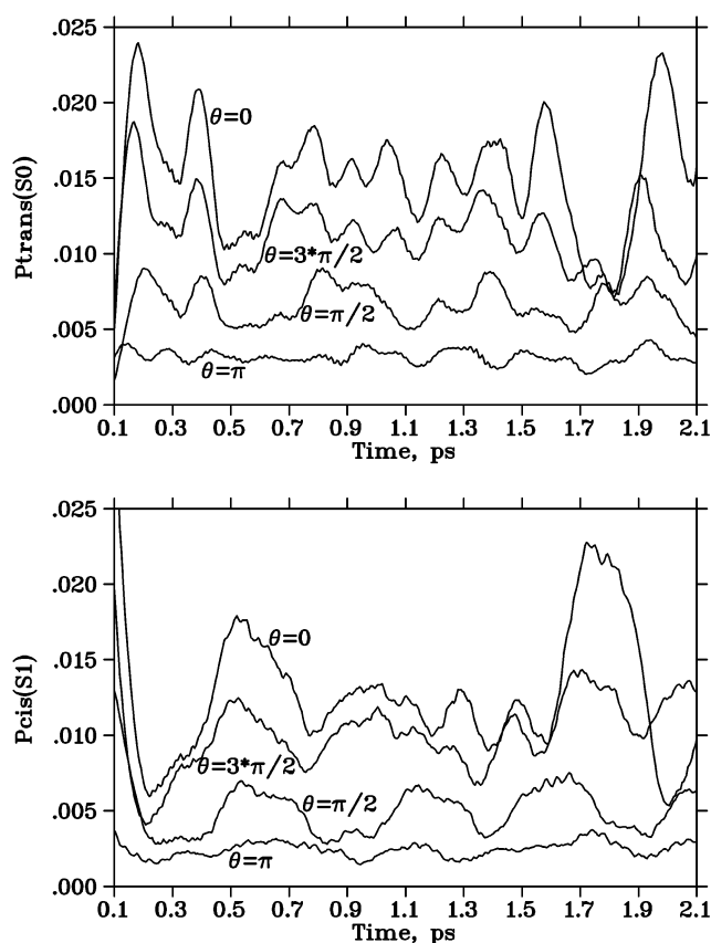
Figure 2. Time-dependent probability of the system to be in the trans configuration of the S_0 electronic state, P_{\text{trans}}^{(S_0)}(t) (upper panel), and the cis configuration of the S_1 electronic state, P_{\text{cis}}^{(S_1)}(t) (lower panel), for relative pump pulse phases \theta = 0, 3\pi/2, \pi/2, and \pi .
